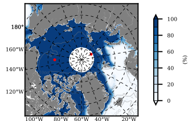
NSIDC mean SICON m09 1991
