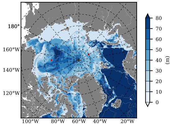
BCTGR273CFSR mean MLD01 over 2002 m03
