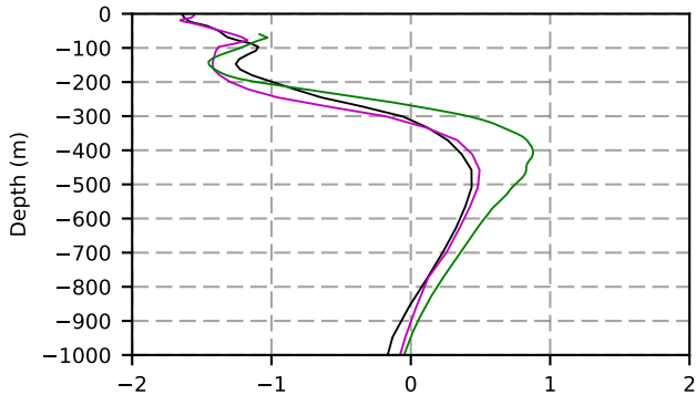
1991 mean temperature @ moor Arctic B box
