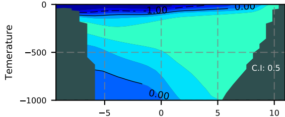
BCTGR273CF SR / FramS Section 1987
