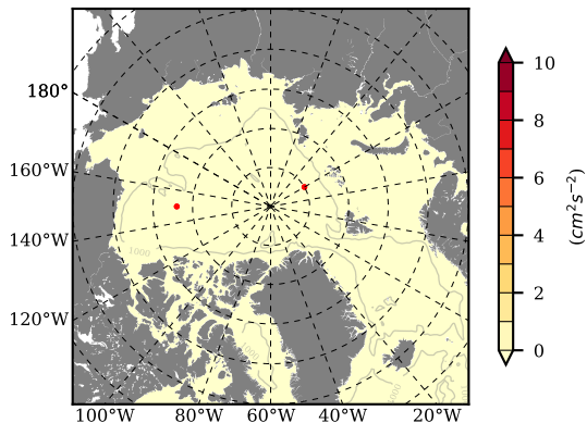
BCTGR273CFSRAO1SC1 mean EKE @ 0 m over 1987
