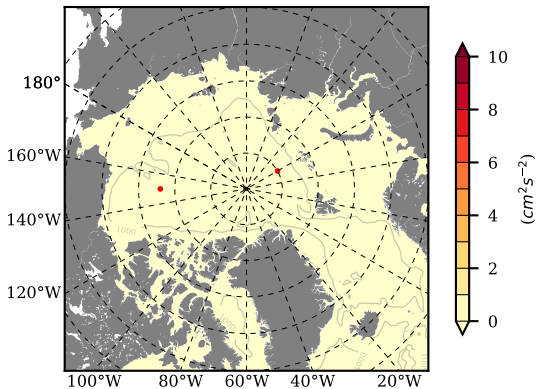
BCTGR273CFSSRAO1SC1 mean EKE @ 0 m over 1990
