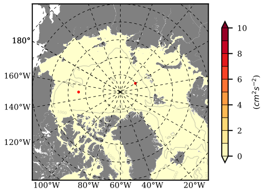
BCTGR273CFRAO1SC1 mean EKE @ 0 m over 2004
