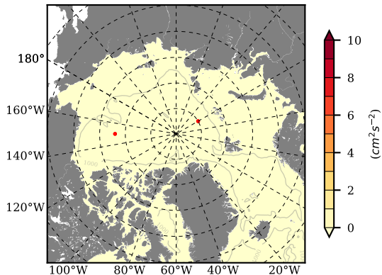
BCTGR273CFSRAO1SC1 mean EKE @ 0 m over 2008
