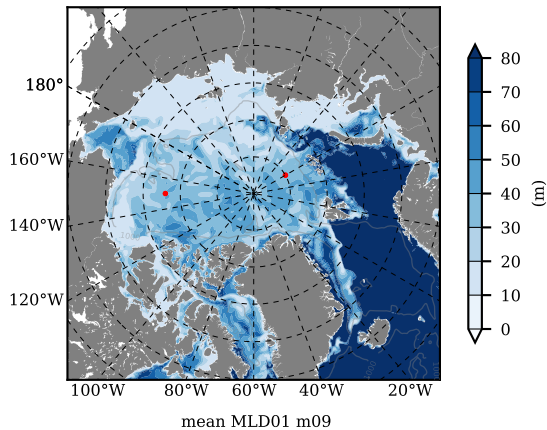
BCTGR273CFSRAO1SC1 mean MLD01 over 1992 m03
