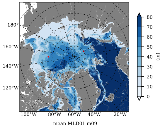
mean MLD01 m09
