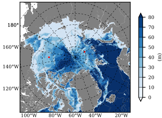
BCTGR273CFSRAO1SC1 mean MLD01 over 1997 m03
