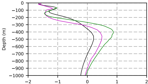
2000 mean temperature @ moor Arctic B box
