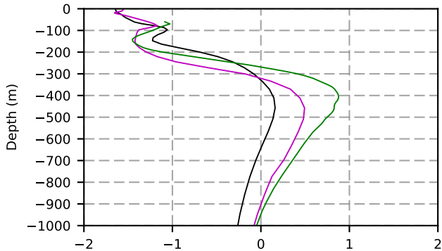
2006 mean temperature @ moor Arctic B box
