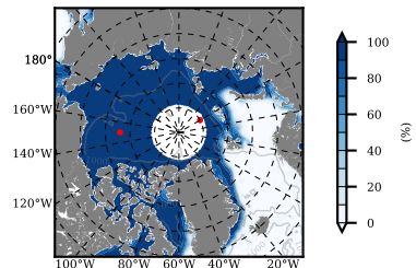
NSIDC mean SICON m09 2006
