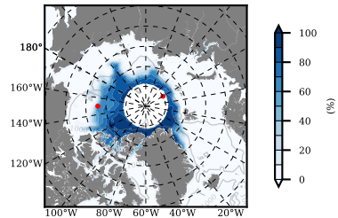
NSIDC mean SICON m09 2014
