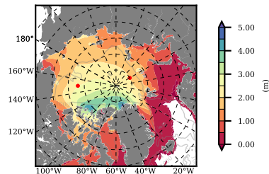
NSIDC mean SICON m03 2014
