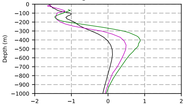
2008 mean temperature @ moor Arctic B box
