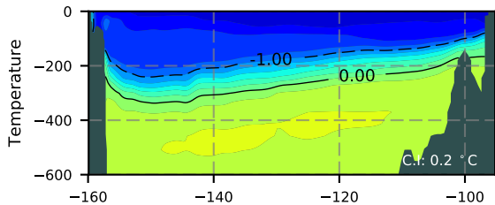
BCTGE28ERA5SC1 / Beaufort Section 1985
