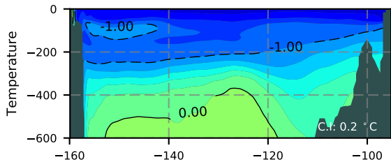
BCTGE28ERA5SC1 / Beaufort Section 2016
