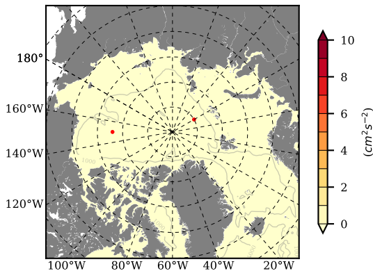
BCTGE28ERA5SC1TPD mean EKE @ 0 m over 1979
