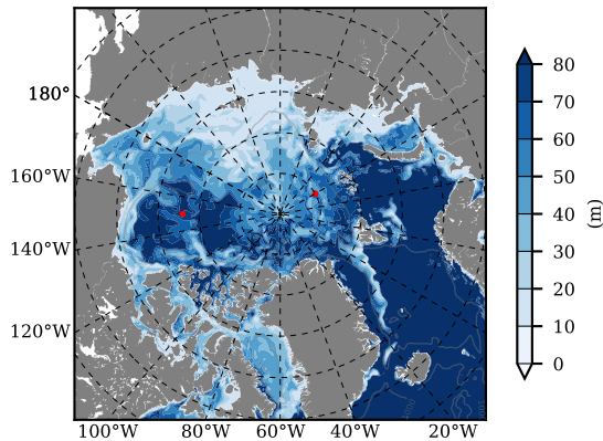
BCTGE28ERA5SC1TPD mean MLD01 over 1986 m03
