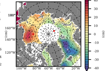
Mean DOT from Armitage et al. 2017 2005
