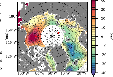
Mean DOT from Armitage et al. 2017 2014
