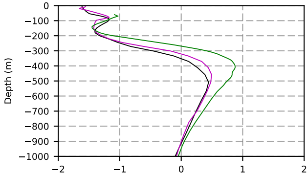
1983 mean temperature @ moor Arctic B box
