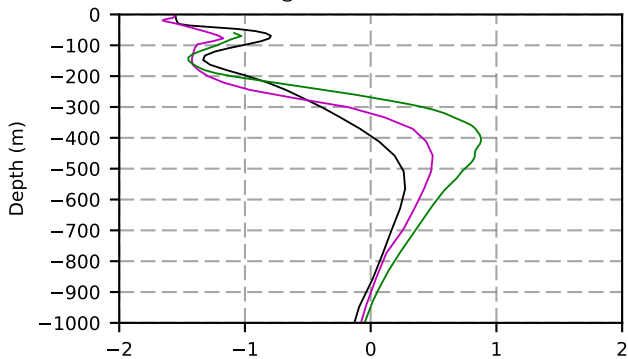
1993 mean temperature @ moor Arctic B box
