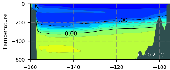
BCTGR273ERA5 / Beaufort Section 1979
