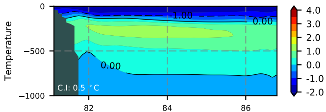
BCTGR273ERA5 / Kara Section 1979
