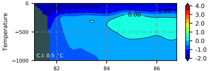
BCTGR273ERA5 / Kara Section 2000
