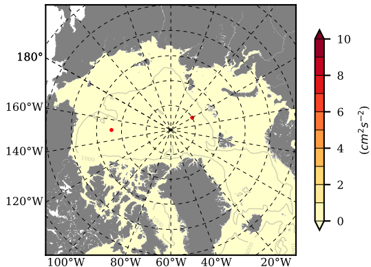
BCTGR273ERA5AO1SC1 mean EKE @ 0 m over 1980
