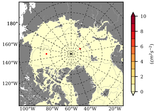
BCTGR273ERA5AO1SC1 mean EKE @ 0 m over 1997
