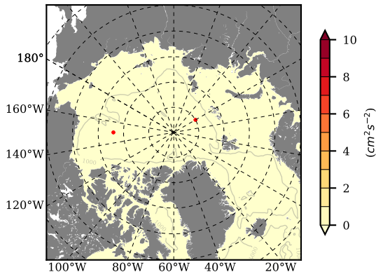
BCTGR273ERA5AO1SC1 mean EKE @ 0 m over 2004
