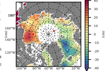
Mean DOT from Armitage et al. 2017 2003
