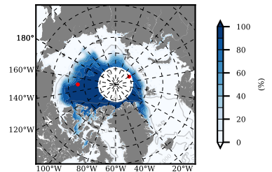
NSIDC mean SICON m09 2004
