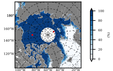
NSIDC mean SICON m09 2004
