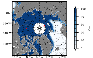
NSIDC mean SICON m09 2008
