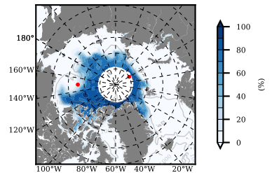
NSIDC mean SICON m09 2008
