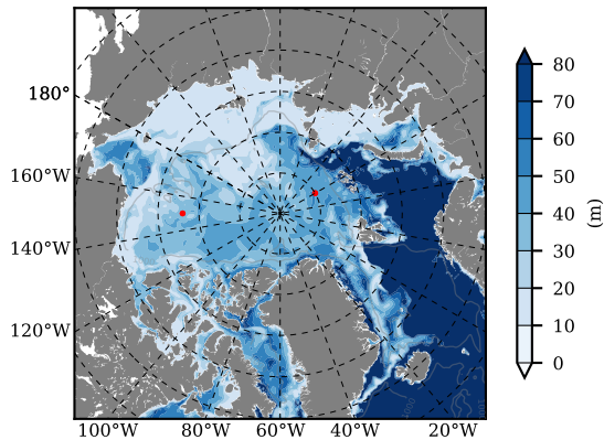
BCTGR273ERA5AO1SC1 mean MLD01 over 1992 m03
