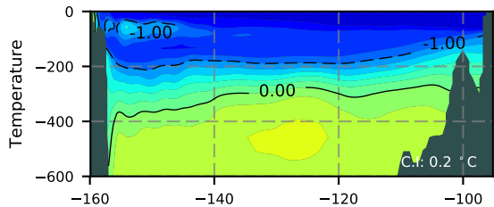
BCTGR273ERA5A01SC1 / Beaufort Section 1993
