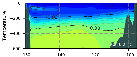
BCTGR273ERA5A01SC1 / Beaufort Section 2000
