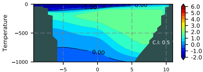
BCTGR273ERA5A01SC1 / FramS Section 1985
