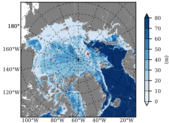
BCTGR273ERA5SC1 mean MLD01 over 1990 m03
