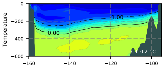
BCTGR273ERA5SC1 / Beaufort Section 1983
