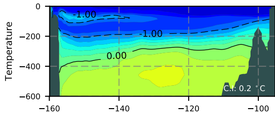
BCTGR273ERA5SC1 / Beaufort Section 1994
