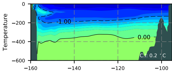
BCTGR273ERA5SC1 / Beaufort Section 2004
