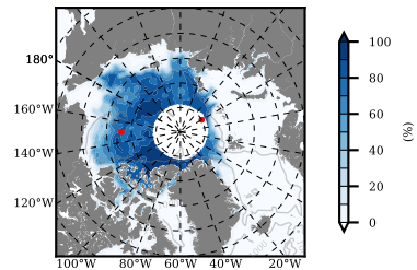
NSIDC mean SICON m09 2000
