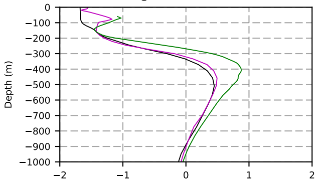
1989 mean temperature @ moor Arctic B box
