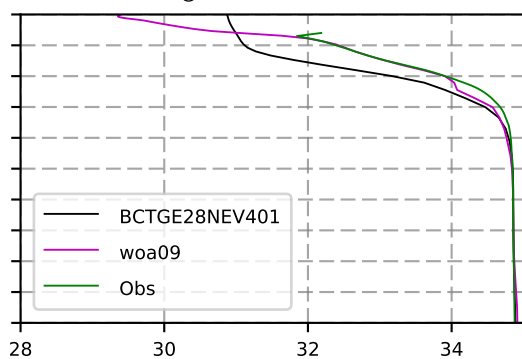
1989 mean Salinity @ moor Arctic B box
