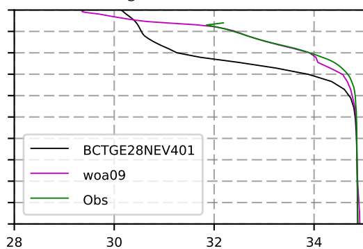
2013 mean Salinity @ moor Arctic B box
