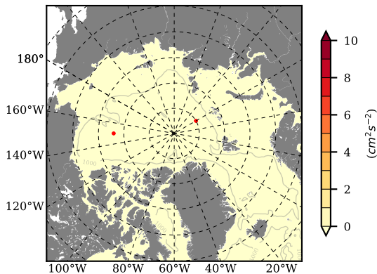
BCTGE28NEV401A1S2 mean EKE @ 0 m over 1985
