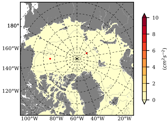
BCTGE28NEV401A1S2 mean EKE @ 0 m over 1987
