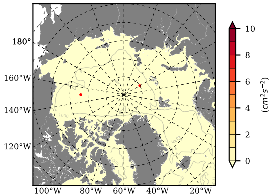
BCTGE28NEV401A1S3 mean EKE @ 0 m over 1984
