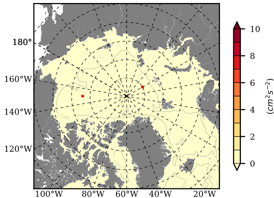
BCTGE28NEV401A1S3 mean EKE @ 0 m over 1996
