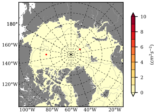
BCTGE28NEV401A1S3 mean EKE @ 0 m over 2010
