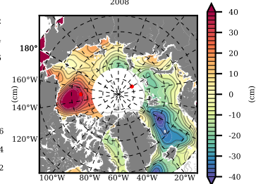
Mean DOT from Armitage et al. 2017 2008
